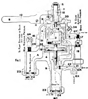
Fig. 2473. Section.
